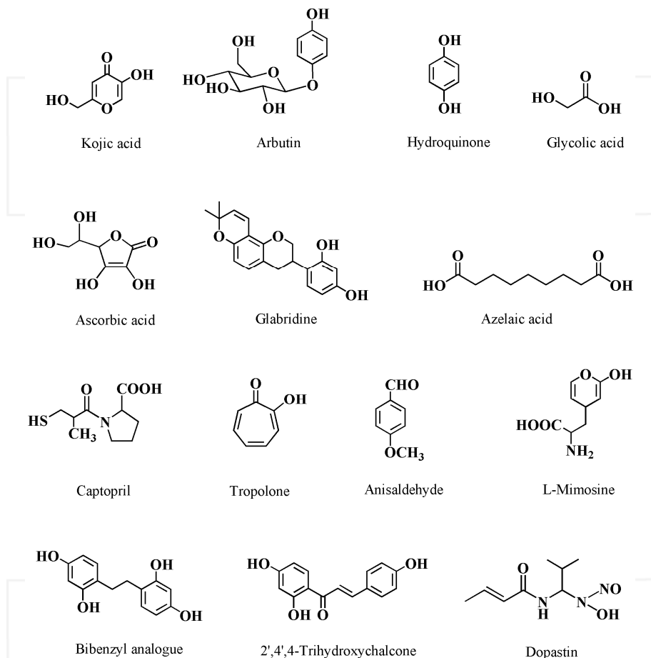
Fig. 1. Some tyrosinase inhibitors.
