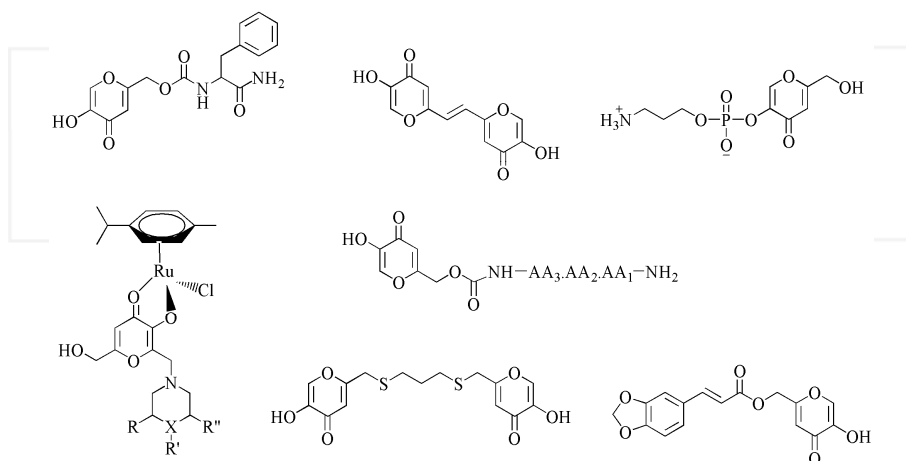
Fig. 3. Chemical structure of some synthetic kojic acid derivatives as tyrosinase inhibitors.
